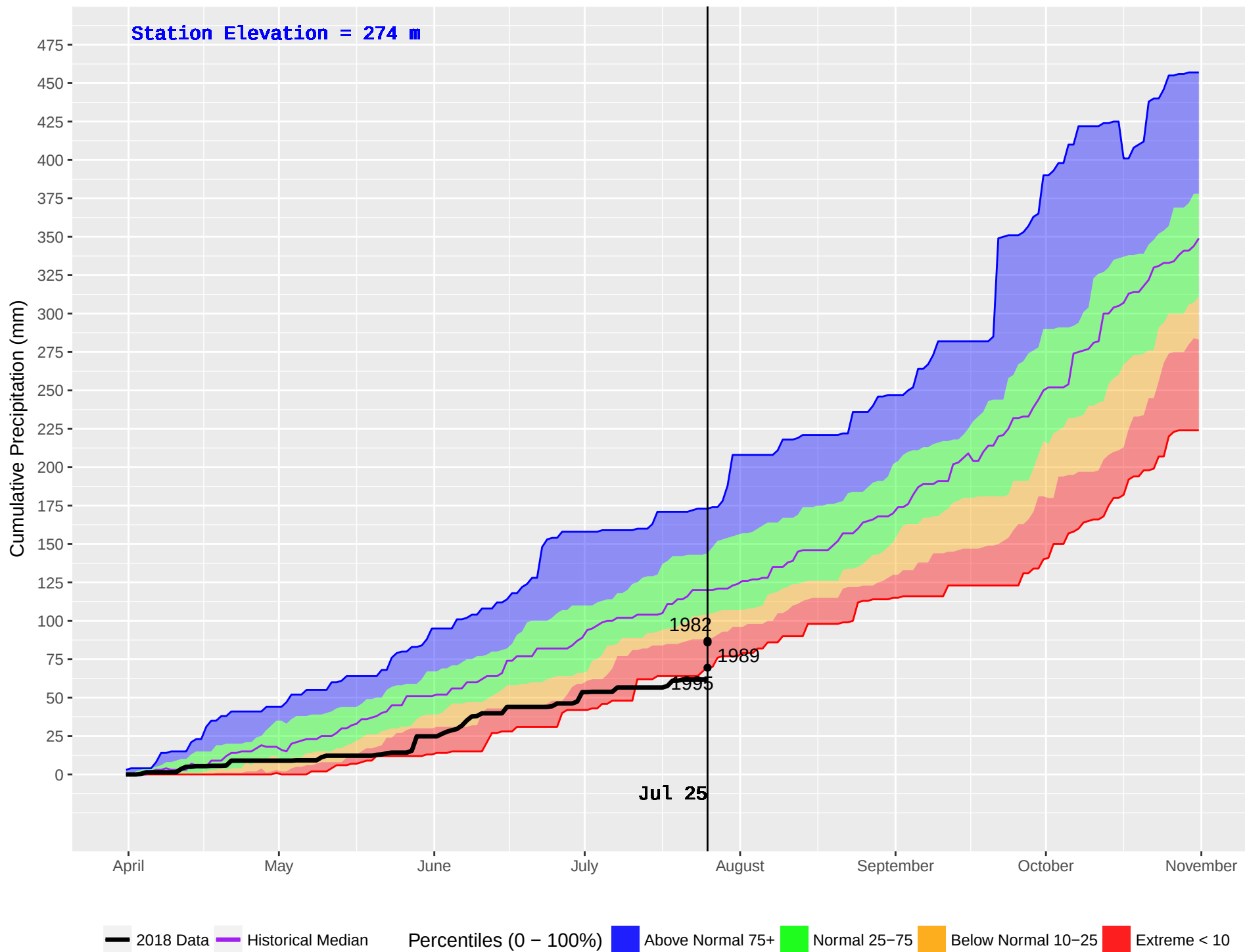
CEDARVALE (429) : Historical (1982–2016) and Current (2018) Noon Cumulative Precipitation
