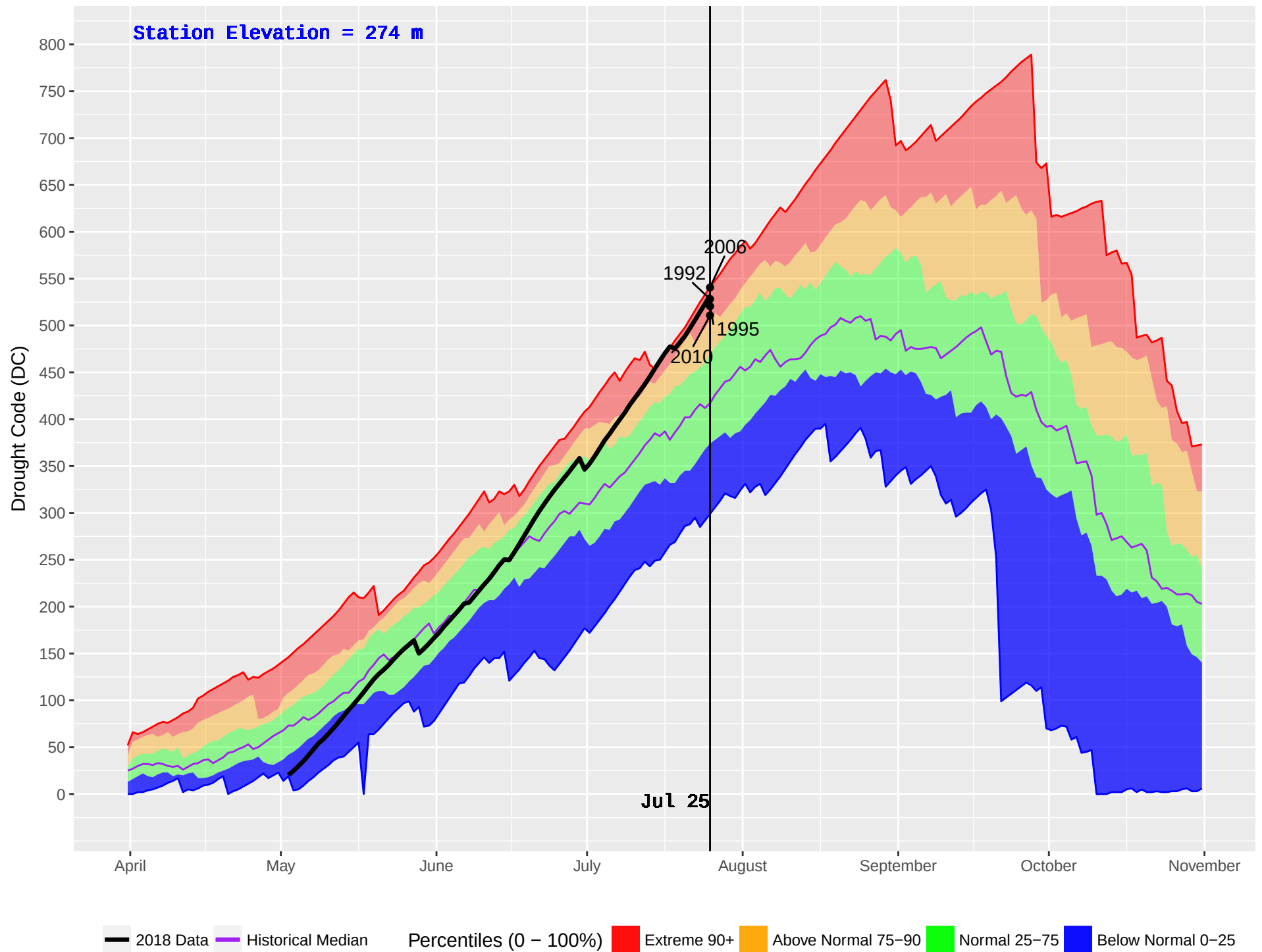
CEDARVALE (429) : Historical (1982–2016) and Current (2018) Noon Drought Code (DC)
